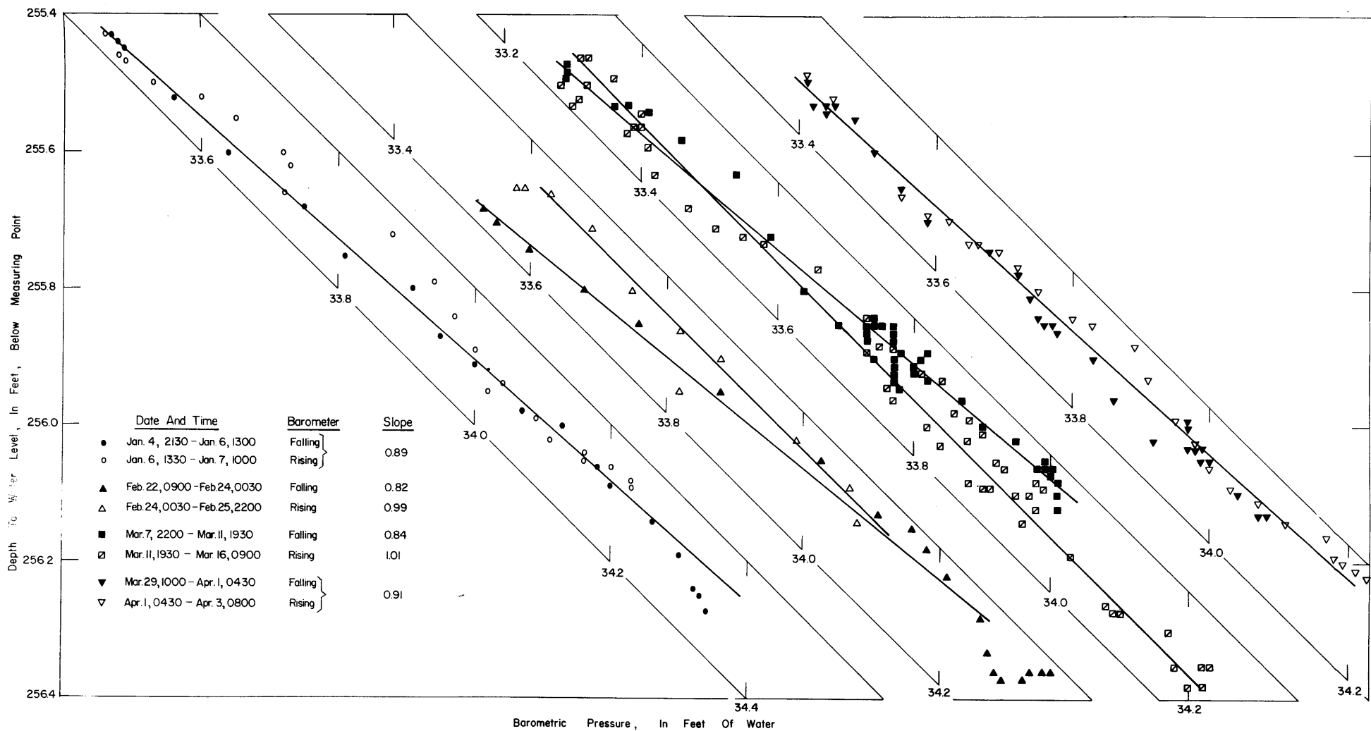
Figure 9. Correlation Between Water Level In University Of Idaho Well No. 3 And Barometric Pressure At Moscow During Selected Periods In 1964
