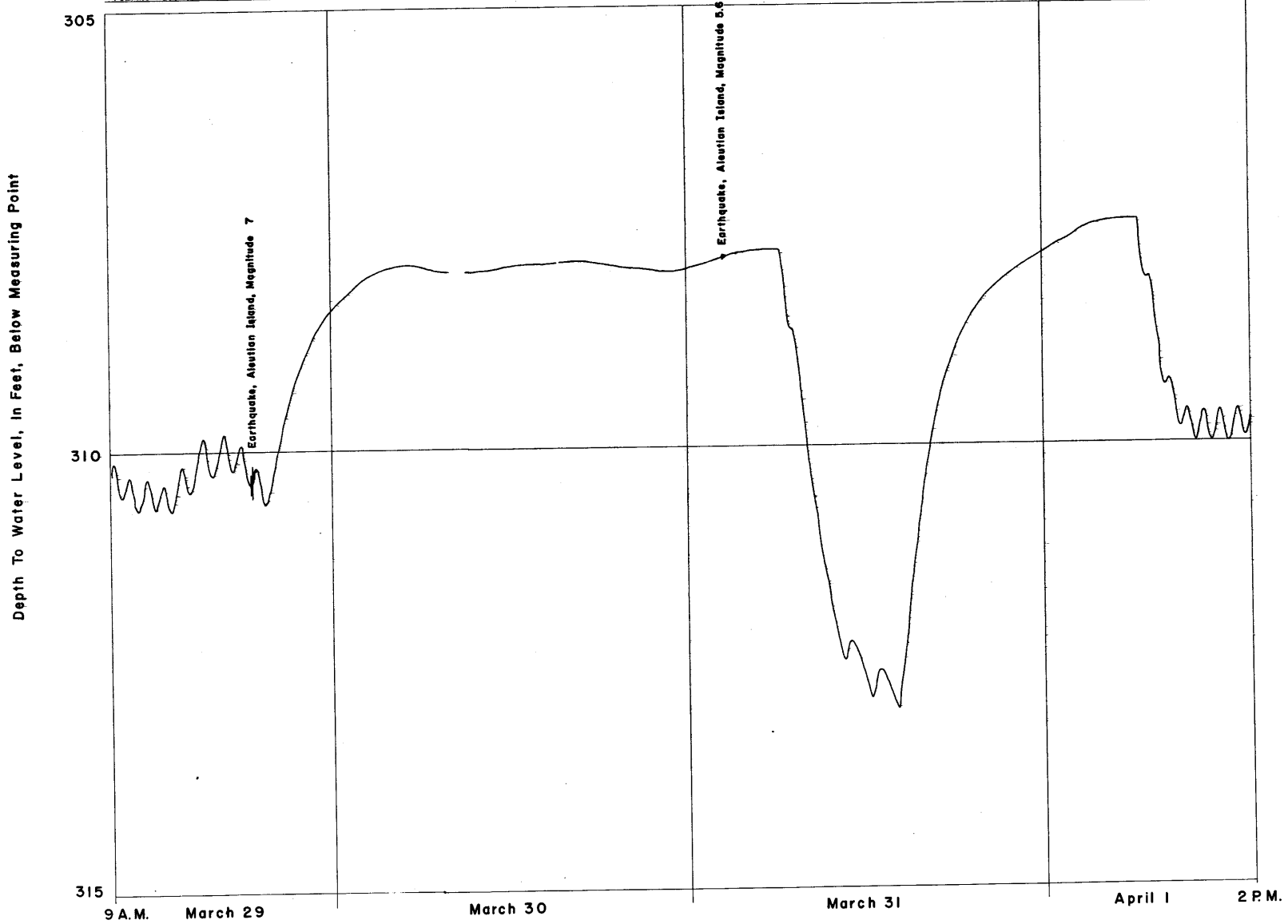
FIGURE 15. HYDROGRAPH OF CITY OF MOSCOW WELL NO. 8, MARCH 29- APRIL 1, 1965
