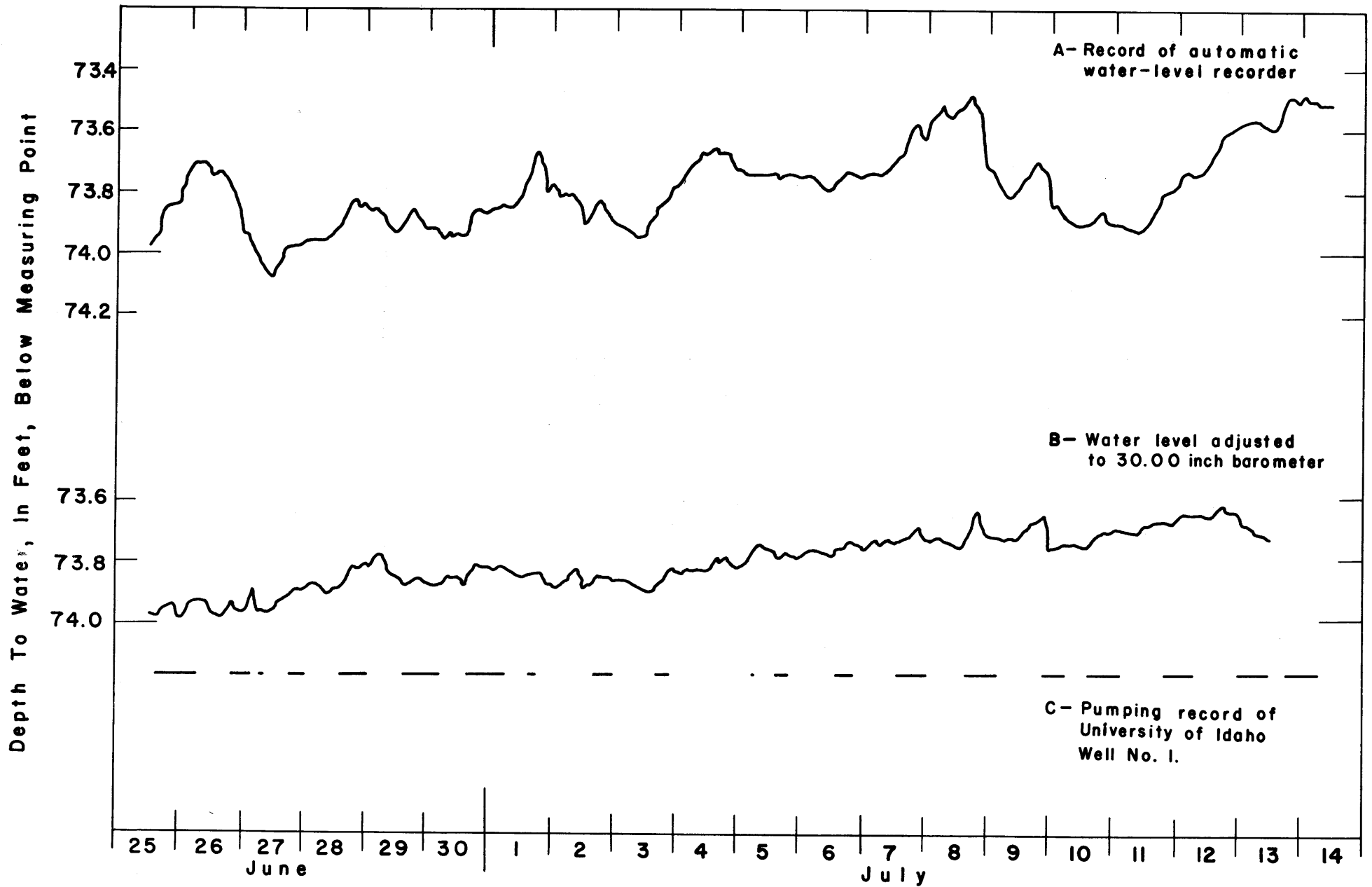
Figure 13. Hydrograph Of University Of Idaho Well No. 2, June 25 - July 14, 1964
