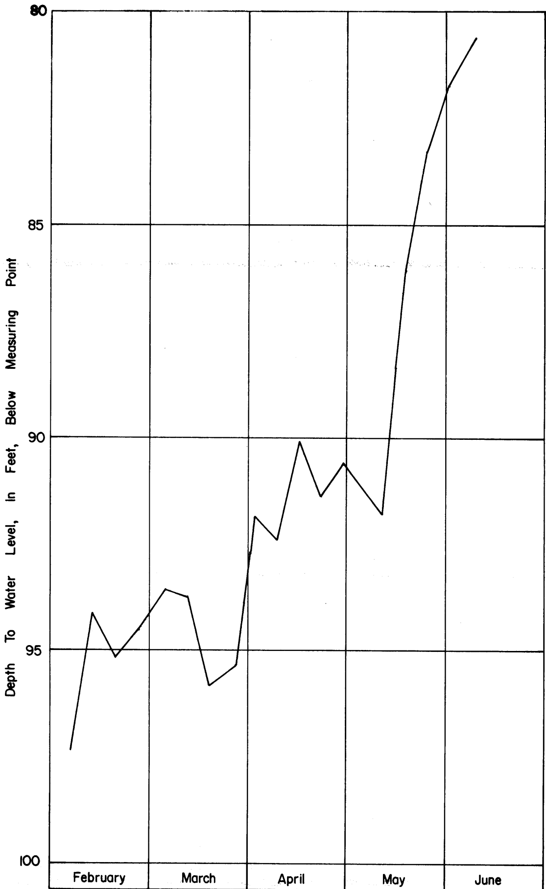
Figure II. Water Level In The 24-Inch casing Of University Of Idaho Well No. 3, February-June 1964
