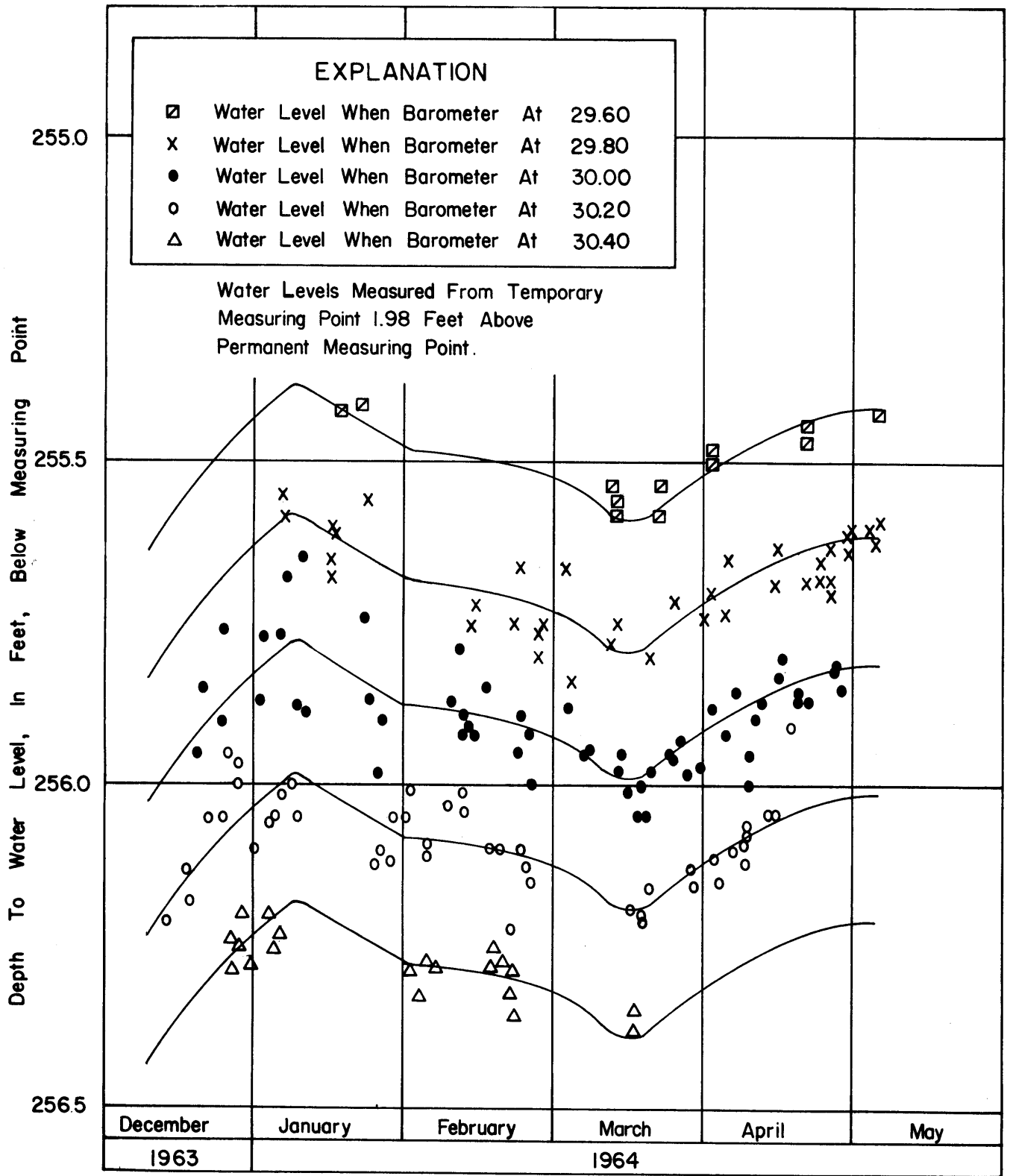
Figure 8. Water Level In University Of Idaho Well No. 3 Coincident With Selected Values Of Barometric Pressure
