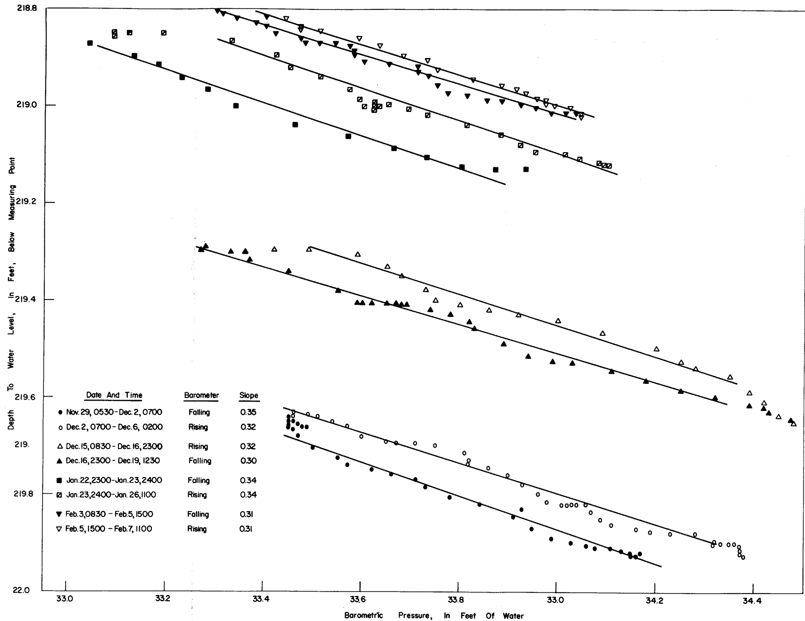
Figure 4. Correlation Between Water Level In City Of Moscow Well No. 7 And Barometric Pressure At Moscow During Selected
