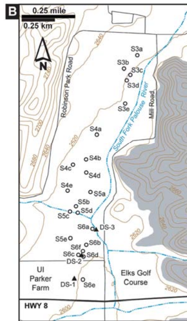
Figure 5: Locations of boreholes within the study areas. Circles indicate shallow borehole locations; triangles are deep boreholes.
